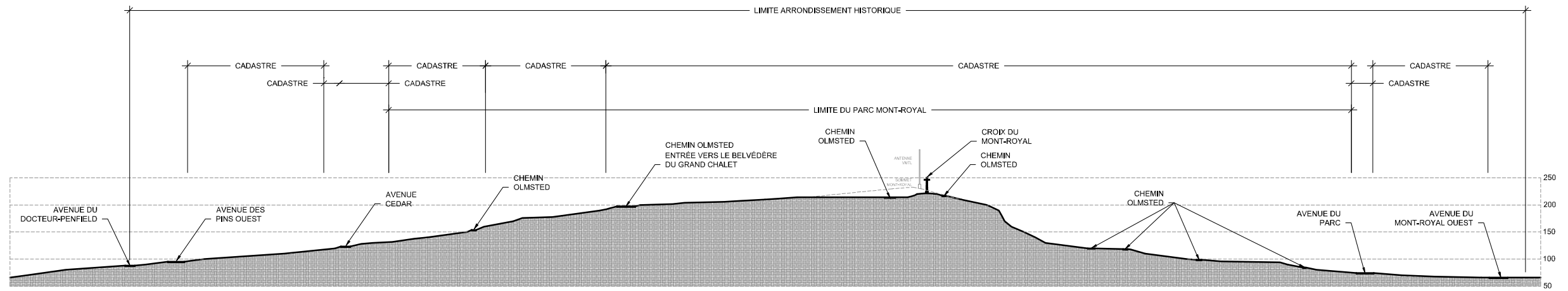
COUPE "C-C"
