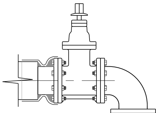
Vidange/Ventouse
